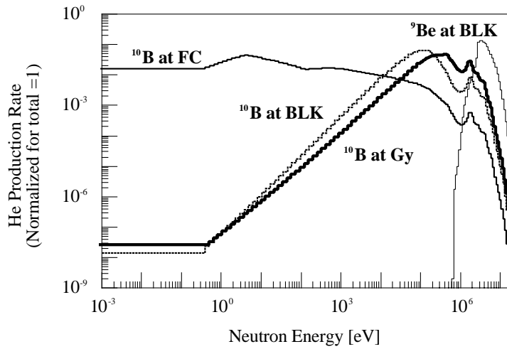
Fig. 3 He Production Rate Spectra
