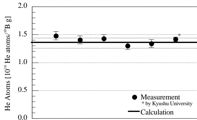
Fig. 4 He Production of B at Glory Hole
