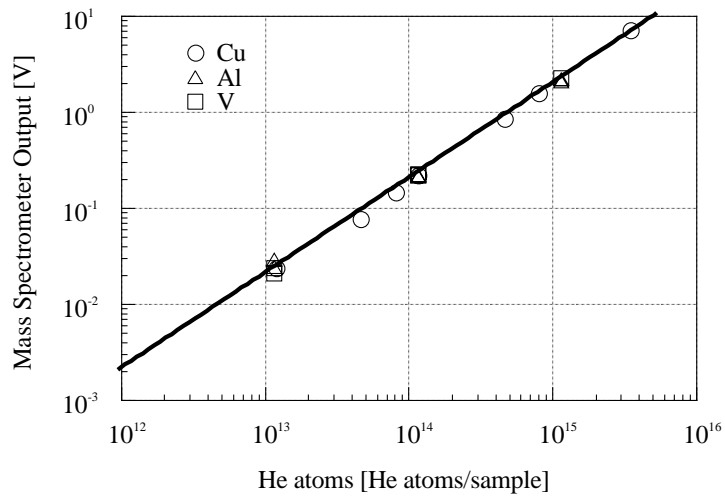
Fig. 2 Calibration Curve
