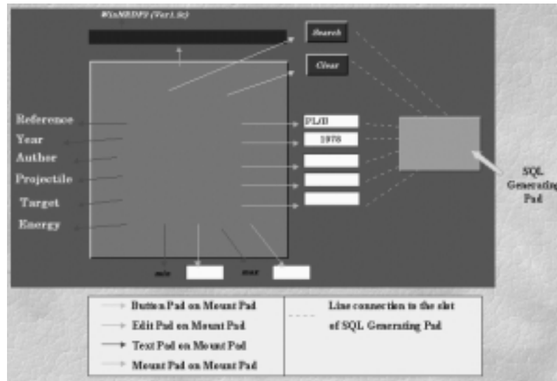
Fig. 5 Decomposition of the query
