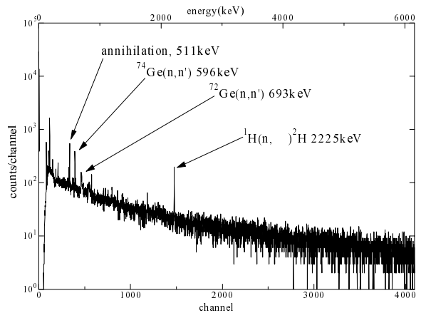
Fig. 6 Foreground spectrum in sample-out system
