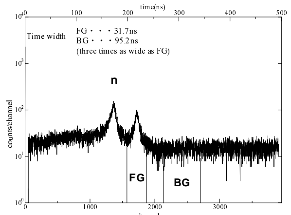
Fig. 4 TOF Spectrum for V-51 with sample-in system
